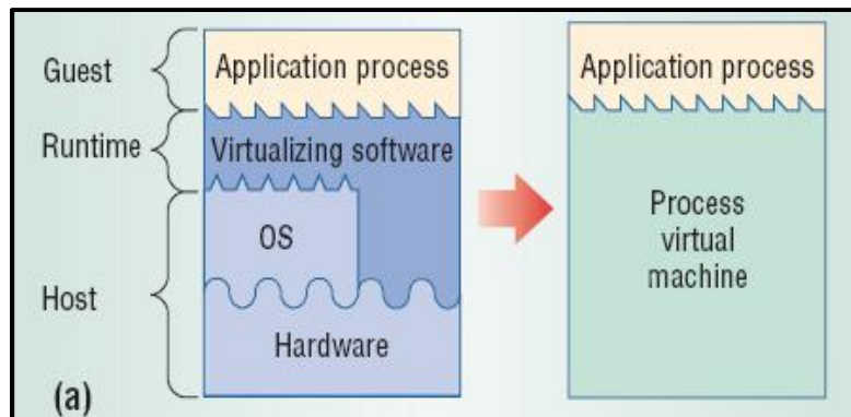
Figure 4: Process VM
