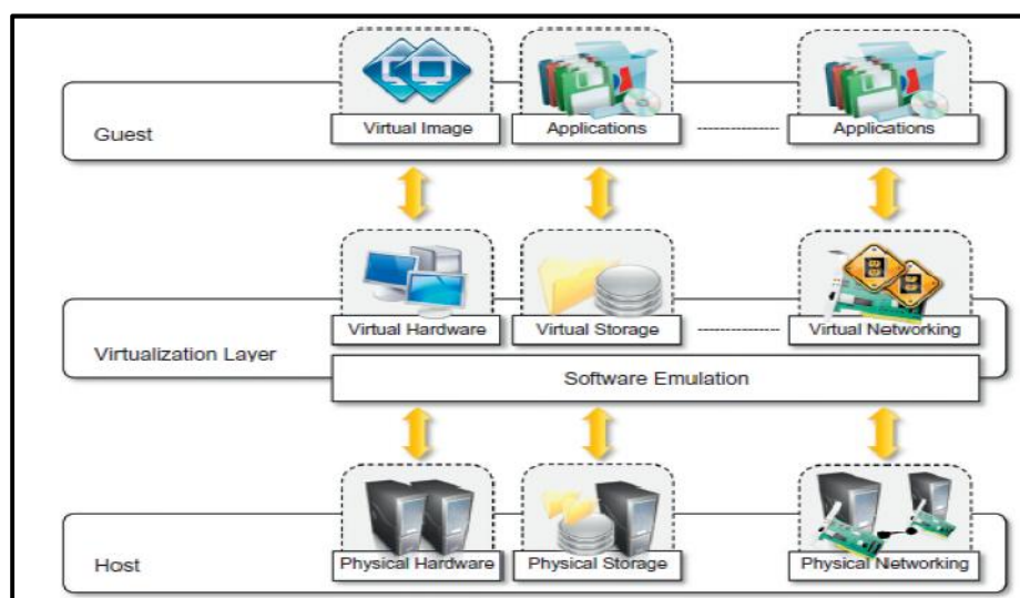
Figure 4: Virtualized Environment
