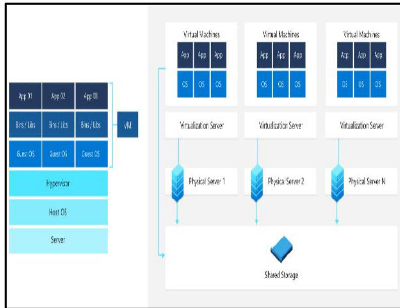
Figure 1: Virtual Machine Scenario
