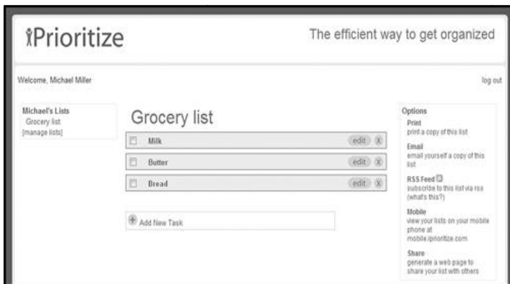
Figure 23: iPrioritize Interface
