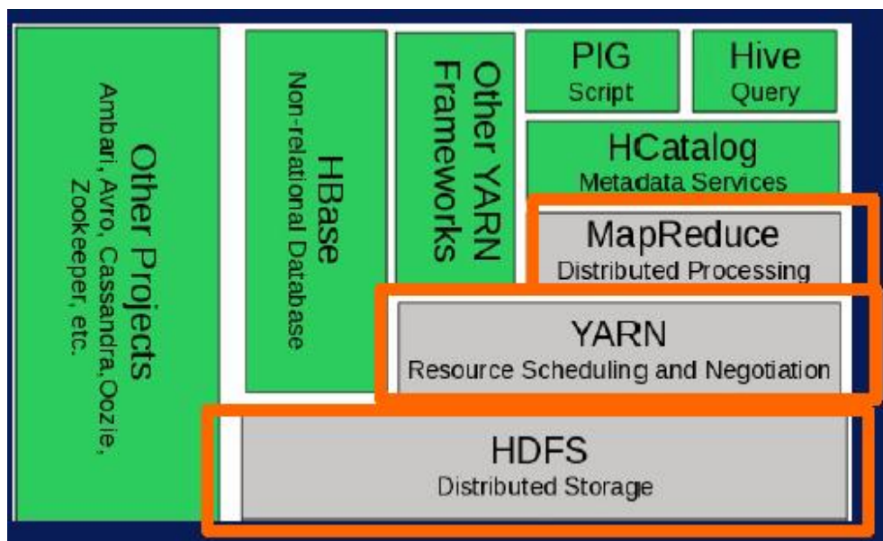
Figure 12: Hadoop Modules
