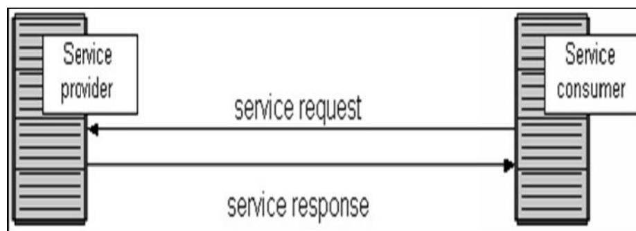
Figure 7: Service-Oriented Architecture
